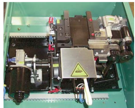
Compact mechanical control head
